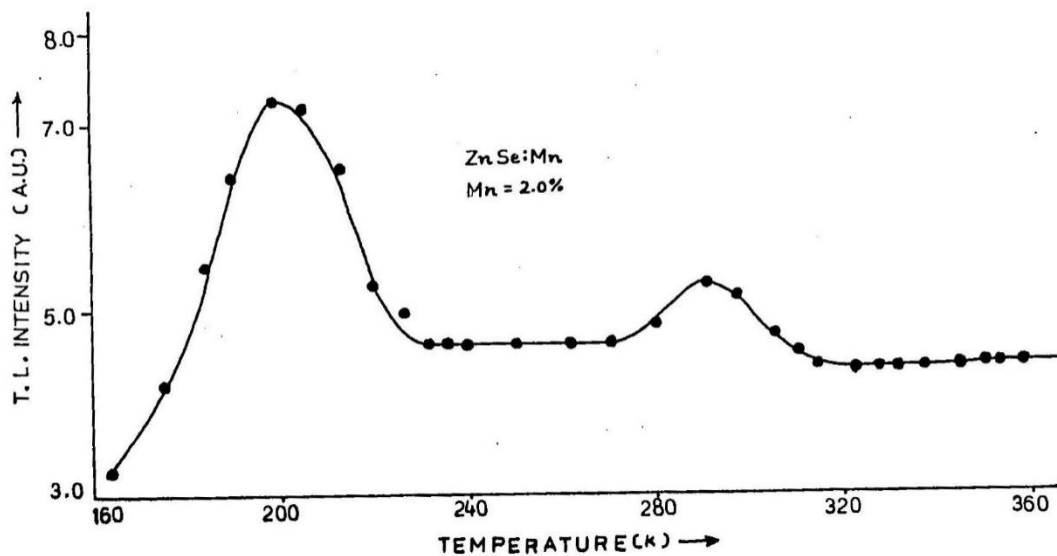
Fig. 1 Glow Curve for ZnSe: Mn
