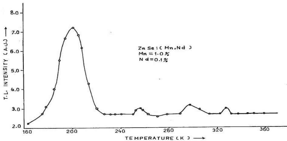
Fig. 2 GLOW CURVE FOR ZnSe:(Mn,Nd) PHOSPHOR
